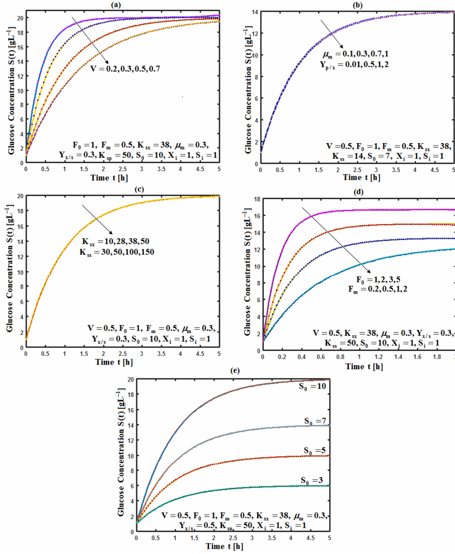
Fig. 3. Concentration profile of glucose versus time for the CMBR Monod. Solid line is the analytical solution given in Eq. (15) and dotted line is the numerical result.
