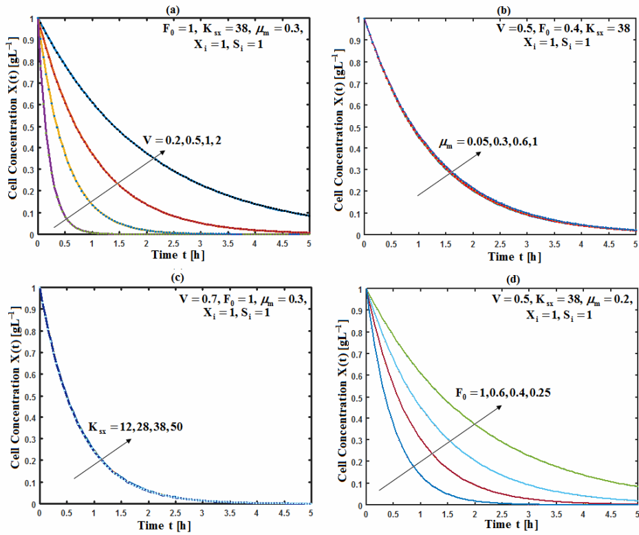
Fig. 5. Profile of concentration of cell growth versus time for CCBR Monod. Solid line is the analytical solution from Eq. (18) and dotted line is the numerical result.
