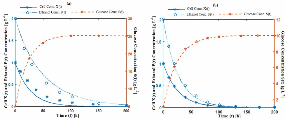
Fig. 1. Concentration profiles of cell growth, glucose consumption and ethanol production. Figure (a) is for the CMBR Monod and Figure (b) is for the CCBR Monod.
