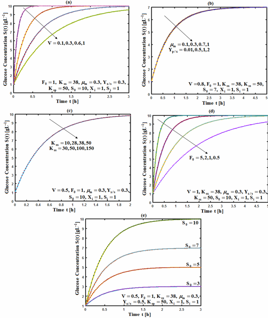
Fig. 6. Profile of concentration of glucose versus time for the CCBR Monod. Solid line is the analytical solution from Eq. (19) and dotted line is the numerical result.
