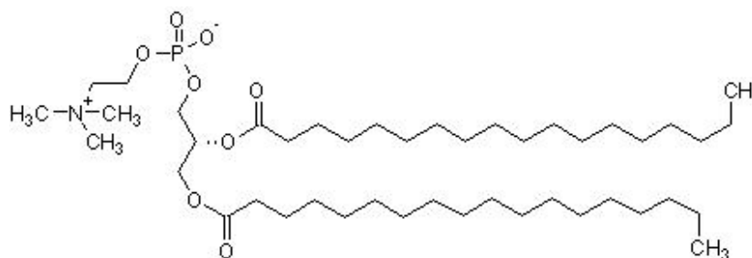
Fig. 2. Schematic chemical structure of DSPC.
