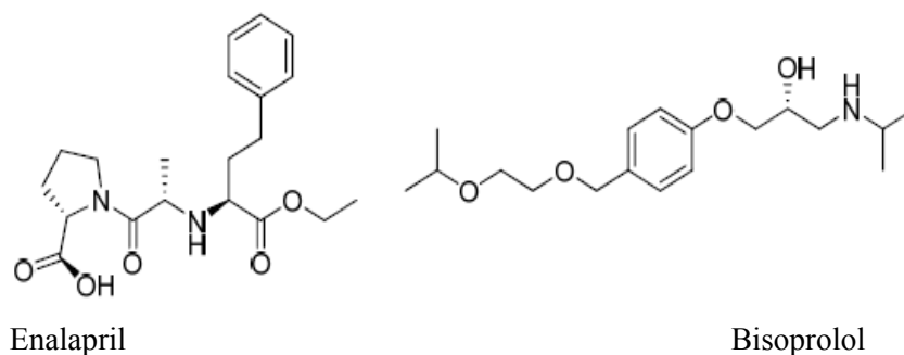
Fig. 1. Schematic chemical structure of enalapril and bisoprolol.
