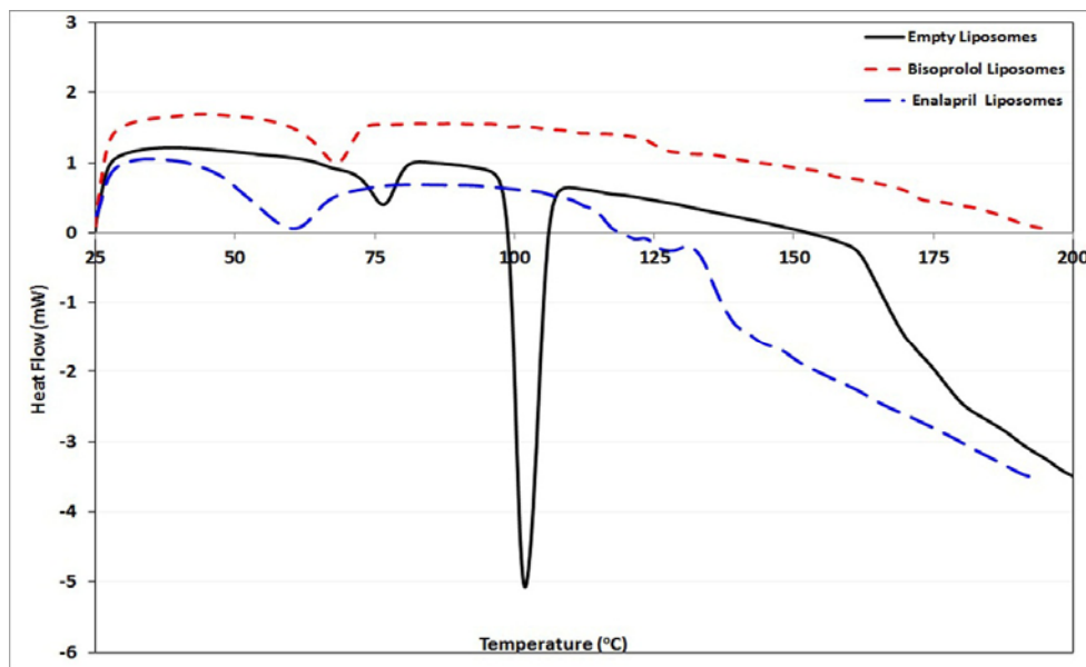
Fig. 3. DSC diagrams of liposomes made of pure DSPC and liposomes doped with bisoprolol or enalapril.
