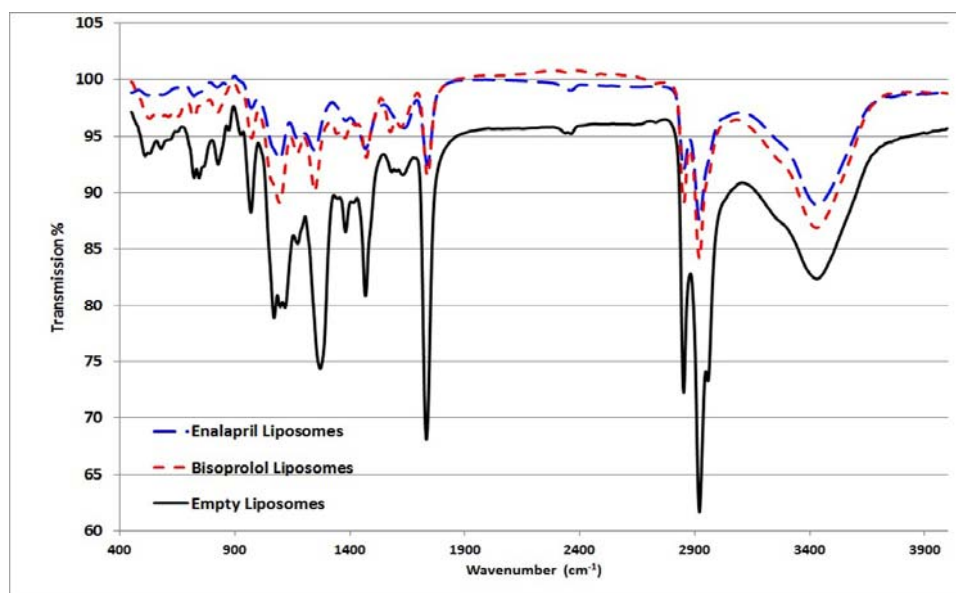
Fig. 4. The full FTIR spectra of empty DSPC and DSPC / bisoprolol or enalapril liposomal samples.
