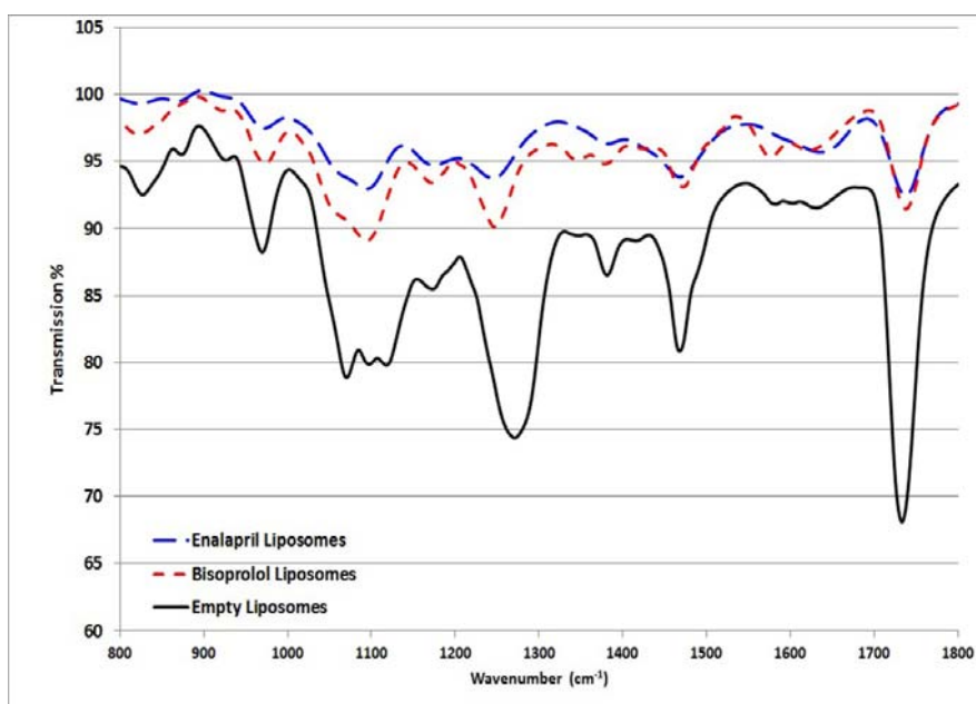
Fig. 6. The magnified part ( 1800\text{--}800\text{ cm}^{-1} ) of FTIR spectra of empty DSPC and DSPC/ bisoprolol or enalapril liposomal samples.
