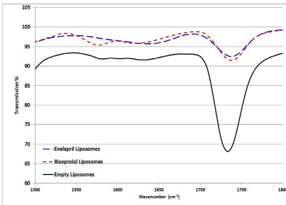
Fig. 7. The magnified part ( 1500\text{--}1800\text{ cm}^{-1} ) of FTIR spectra of empty DSPC and DSPC / bisoprolol or enalapril liposomal samples.
