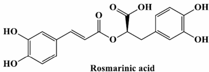
Fig. 1. Chemical structure of rosmarinic acid.
