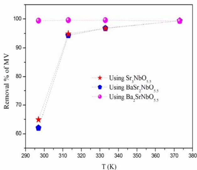
Fig. 5. the effect of temperature on the MV removal. The time, volume, pH and concentration of dyes solutions are 150 min, 50 mL, 5.1 and 10 ppm, respectively.
