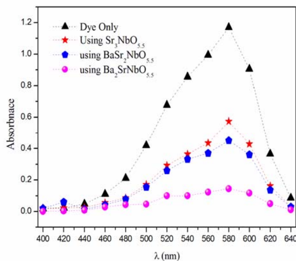
Fig. 3. The wavelength dependence of absorbance for MV solution. The time, volume, concentration, adsorbent mass and pH of MV solution are 150 min, 50 mL, 10 ppm, 0.1 g and 5.1, respectively.
