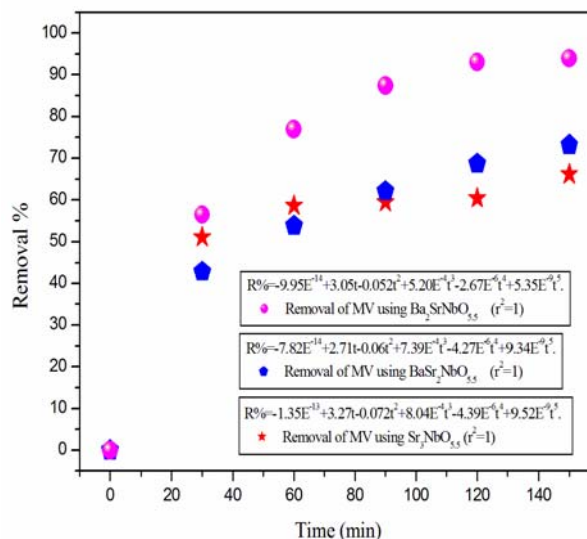
Fig. 2. The time dependence of MV removal at room temperature. The volume, concentration, and pH of the dye solution are 50 mL, 10 ppm and 5.1, respectively. E is the Langmuir constant and r^2 is the correlation coefficient.
