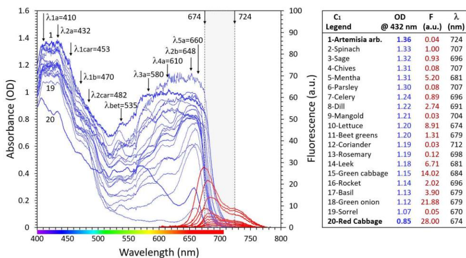
Fig. 1. Optical absorption spectra (blue curves) and fluorescence spectra (red curves) of the as extracted solutions concentrations – C1 (9–15 \mu\text{g}/\text{cc} ). The OD in the annexed table is given in decreasing order and together with the black numbers above or below the absorption curves aid in the identification of the specific plant absorbance curve.
