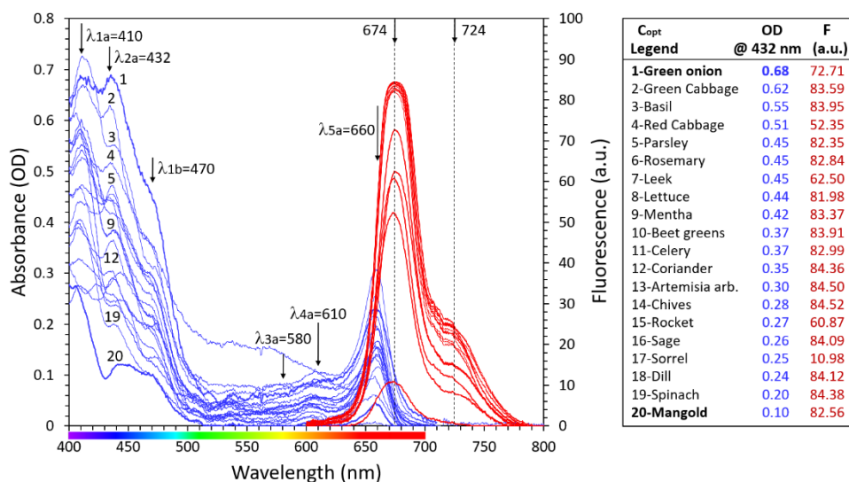
Fig. 2. Optical absorption spectra (blue curves) and fluorescence spectra (red curves) of all plant solutions at optimal Chl-a concentrations – C_{opt} (1–7 \mu\text{g}/\text{cc} ). The OD decreasing values in the table together with the black numbers above the absorption curves aid to identify the specific plant curve.
