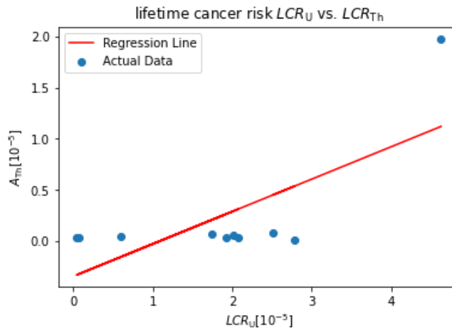
Fig. 5. Excess lifetime cancer of adults due to ^{232}\text{Th} vs. that of ^{238}\text{U} whose relation is given by LCR_{\text{Th}} = 0.316 LCR_{\text{U}} - 0.344 and r^2 = 0.51 of tea leaves from Gumero farm for adults.
