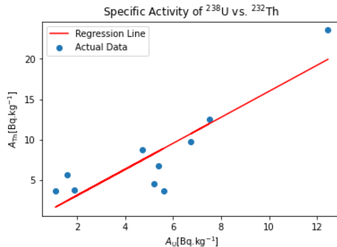
Fig. 3. The specific activity of ^{232}\text{Th} vs. ^{238}\text{U} whose relation is given by A_{\text{Th}} = 1.61A_{\text{U}} - 0.115 with root mean square error (RMSE) 0.78.
