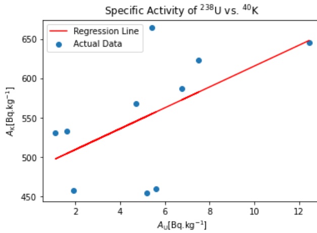
Fig. 4. The specific activity of ^{40}\text{K} vs. ^{238}\text{U} whose relation is given by A_{\text{K}} = 13.23 A_{\text{U}} + 483.41 , and r^2 = 0.32 . It was considered that 1 L of liquid tea has a mass of 1 kg.
