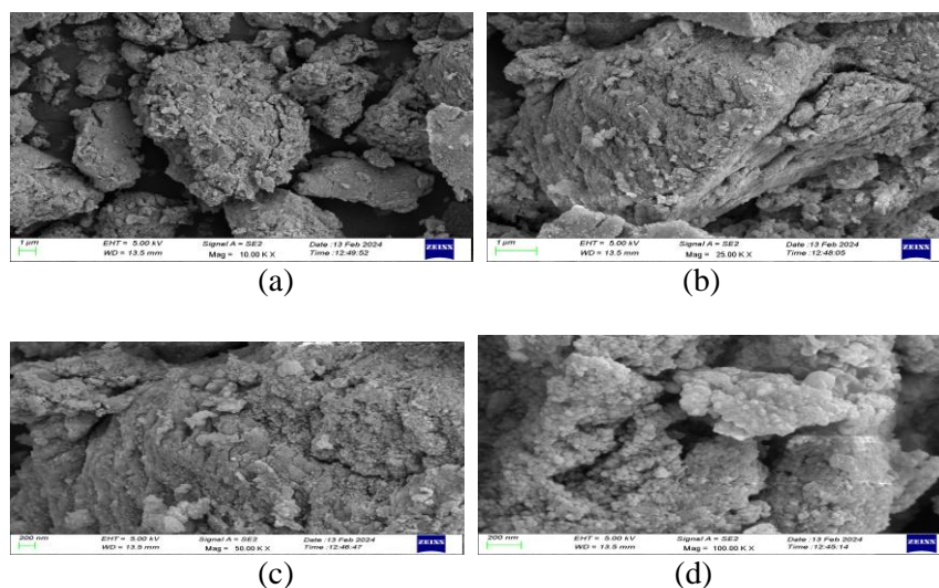
Fig. 15. FESEM imaging of cinnamon-based synthesized silver nanoparticles at: a) 10 KX; b) 25 KX; c) 50 KX; d) 100 KX.
