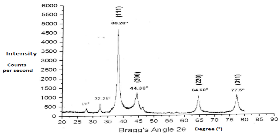
Fig. 12. XRD crystallography of silver nanoparticles of sample \text{AgNO}_3 + cinnamon.
