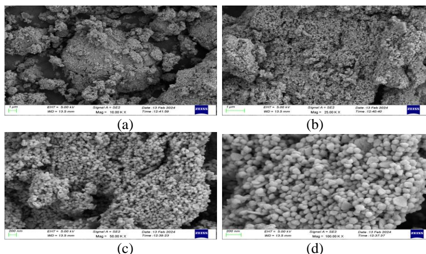
Fig. 13. FESEM imaging of cloves-based synthesized silver nanoparticles at: a) 10 KX; b) 25 KX; c) 50 KX; d) 100 KX.
