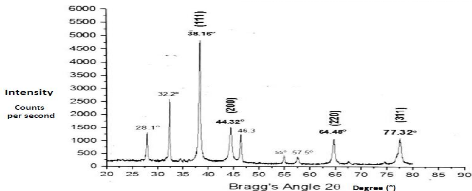
Fig. 11. XRD crystallography of silver nanoparticles of sample \text{AgNO}_3 + clove.
