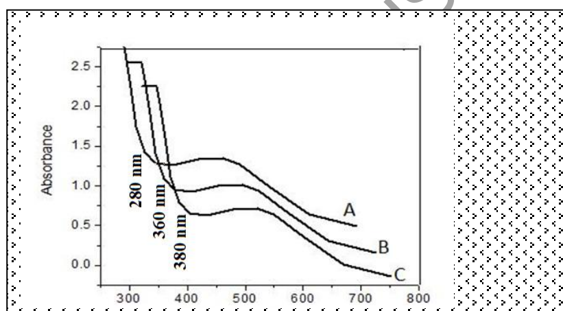
Fig. 6. UV-Vis absorption spectrum of Fe doped ZnS/CdS nanoparticle.
