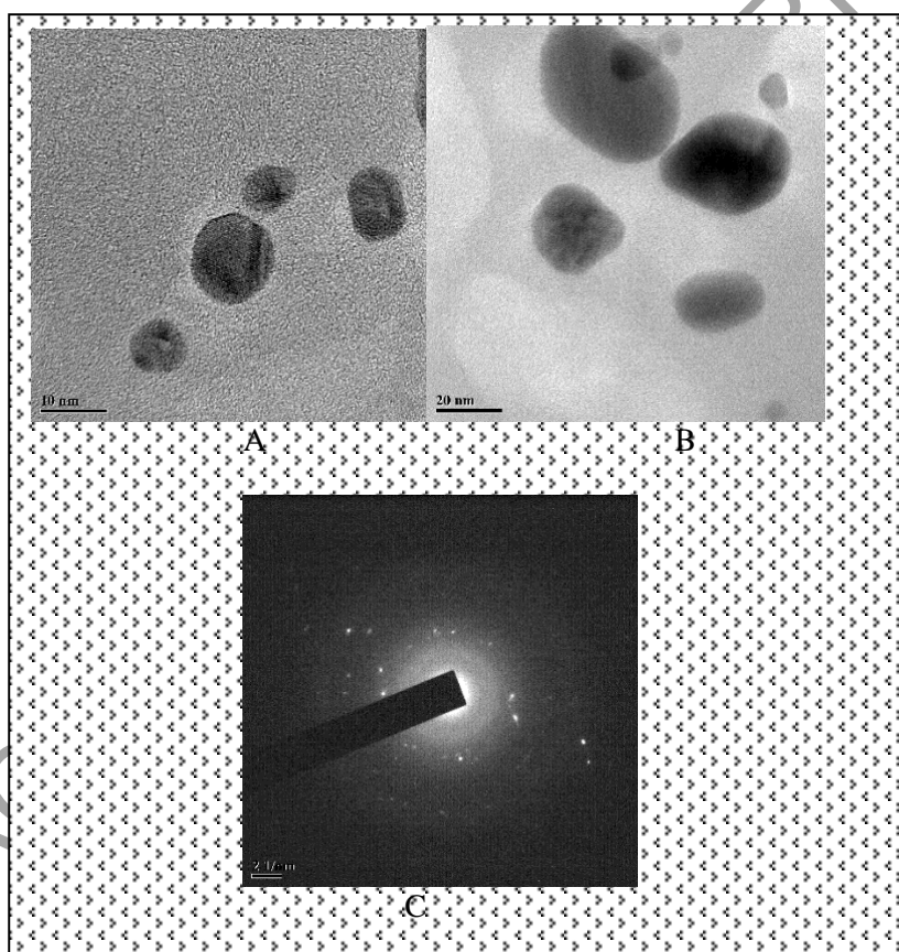
Fig. 2. TEM micrograph of ZnS/CdS nanoparticle (A) without doping, (B) after Fe doping, and (C) SAED pattern of the one-dimensional Fe doped ZnS/CdS.
