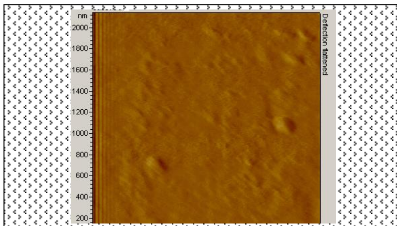
Fig. 4. 2D AFM image at 2.0 wt% Fe-doped ZnS/CdS nanoparticles.
