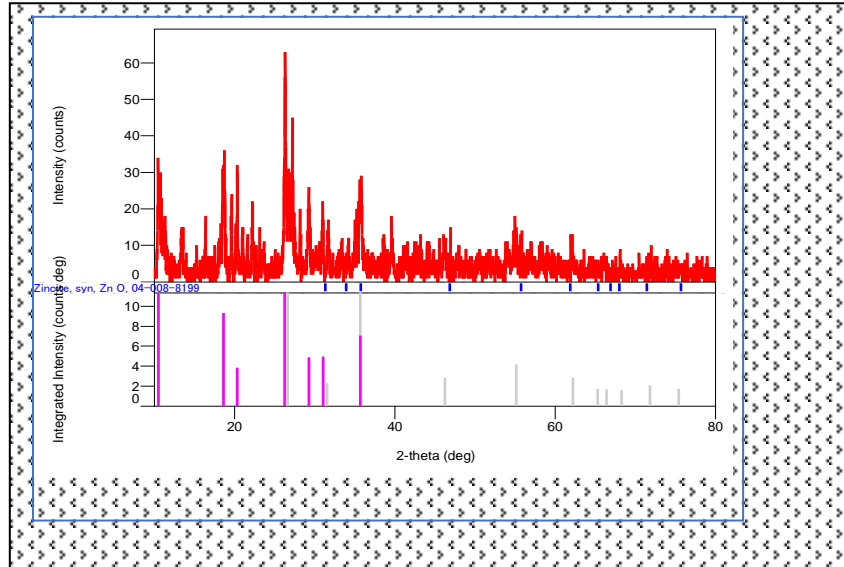
Fig. 1. XRD Rietveld refinement spectrum of Fe doped ZnS/CdS.
