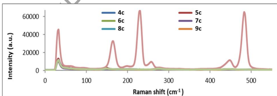
Fig. 3. Raman spectra of potentized samples from 4c–9c, pure sulphur, and pure ethanol.
