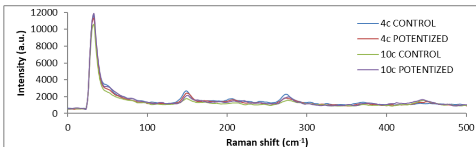
Fig. 4. Comparison of Raman spectra of control and potentized samples of 4c and 10c for sulphur region.
