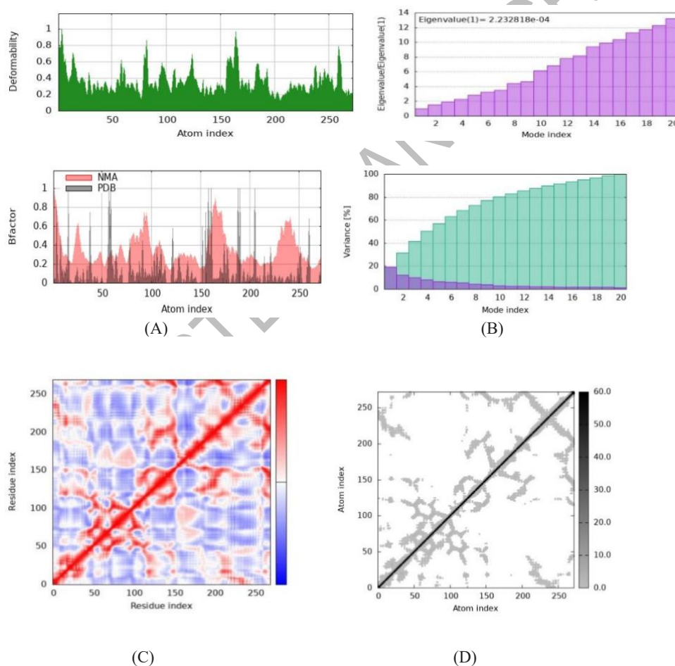
Fig. 5. Outputs of molecular dynamics simulations in iMODS (A) deformability
