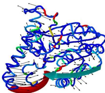
Fig. 4. Molecular mobility evaluated by NMA of the docked complex.
