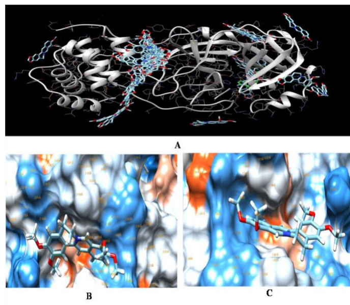
Fig. 5. The docking studies visualized in UCSF Chimera software were (A) the total available clusters are depicted upon binding with target molecule, (B) depicted interaction of ligand palmatine in vicinity with eight sites, (C) insight of most thermodynamically stable cluster rank 2 palmatine H-bond distance with target.
