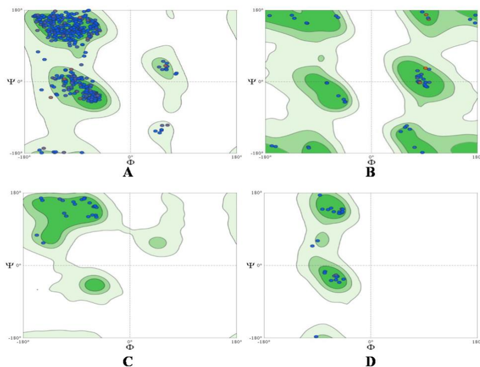
Fig. 2. Ramchandran plot obtained using MolProbity for overall protein (A) and for glycine (B), preproline (C), and proline (D) amino acids.
