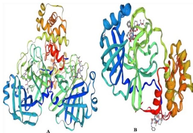
Fig. 3. SWISS-MODEL Structure (A) predicted the 3-dimensional structure of COVID-19 main protease and (B) superior structural alignment with different templates.
