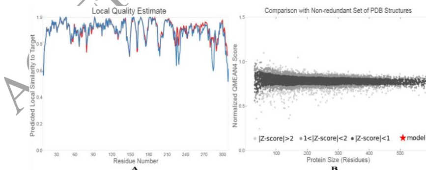
Fig. 4. The two criteria depicted for structural assessments are (A) local quality estimate and (B) comparison with non-redundant set of PDB structures.
