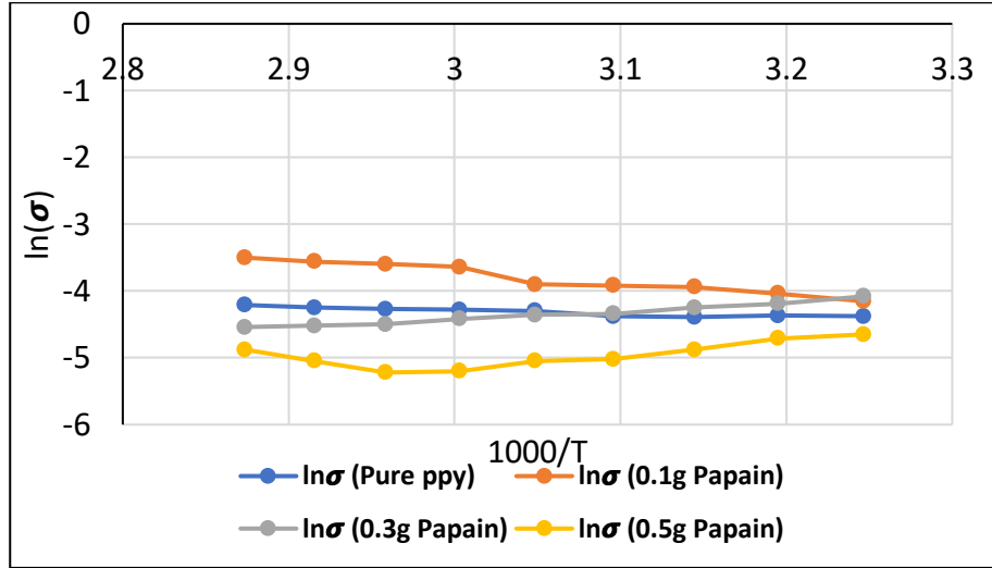
Fig. 4. Plot of \ln(\sigma) vs 1000/T for pure ppy and ppy doped with small amounts of papain.
