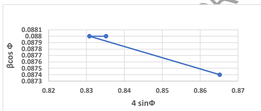
Fig. 1. W-H plot of papain-ppy composite doped with 0.1, 0.3, 0.5 g of papain.
